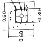
PEDESTAL DETAILS
